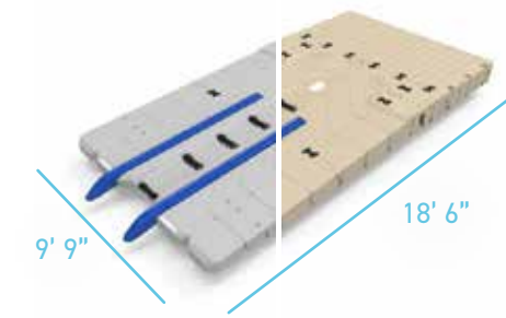
EZ BoatPort with Side Extensions & Large Platform 190 sf BP3001-EZGR, BP3001
