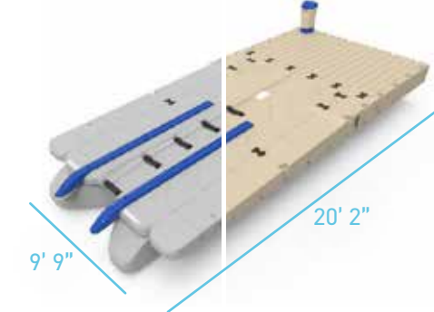
EZ BoatPort with Side Extensions, Float Tank, & Air Assist 205 sf BP5000-EZGR, BP5000
