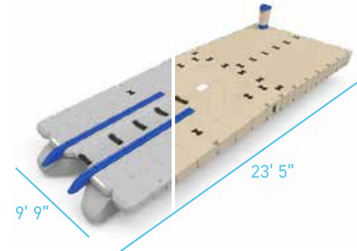
EZ BoatPort with Side Extensions, Float Tank, Air Assist, & Large Platform 240 sf BP5001-EZGR, BP5001
